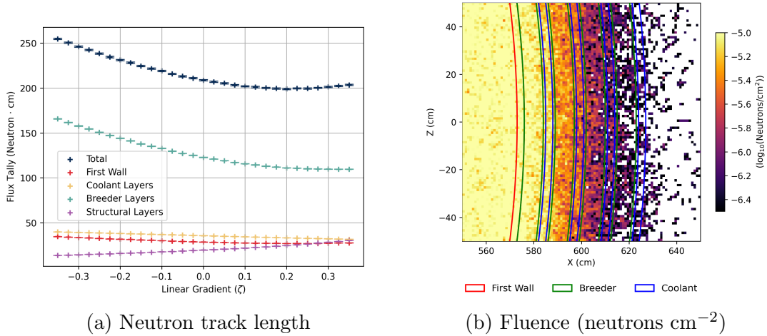
Figure 12: These figures demonstrate how neutron transport changes in the blanket. The effect of \zeta on the neutron track length measured by the ‘flux’ tally is shown in figure a. Figure b demonstrates the exponential decay of fluence throughout a 2D slice of the breeder.
