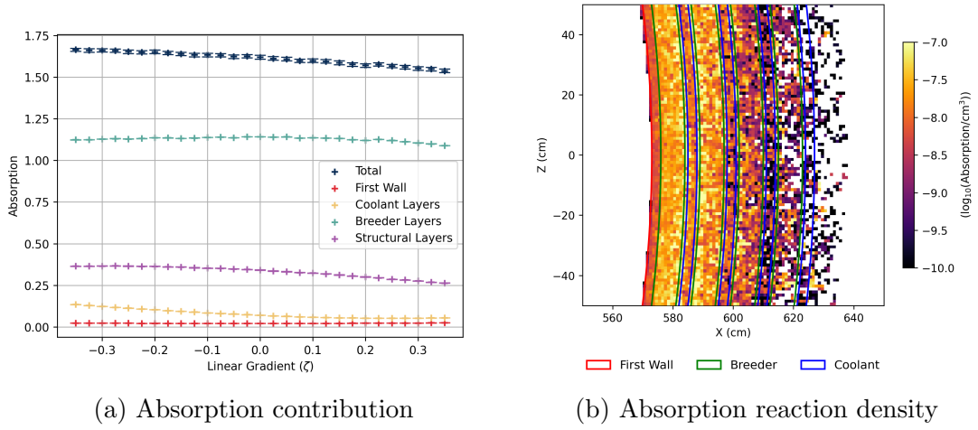
Figure 8: Two graphs showing the absorption measured in the breeder blanket. A graph of absorption at several \zeta values is shown in figure a with a 2D heat map of the absorption in figure b.
